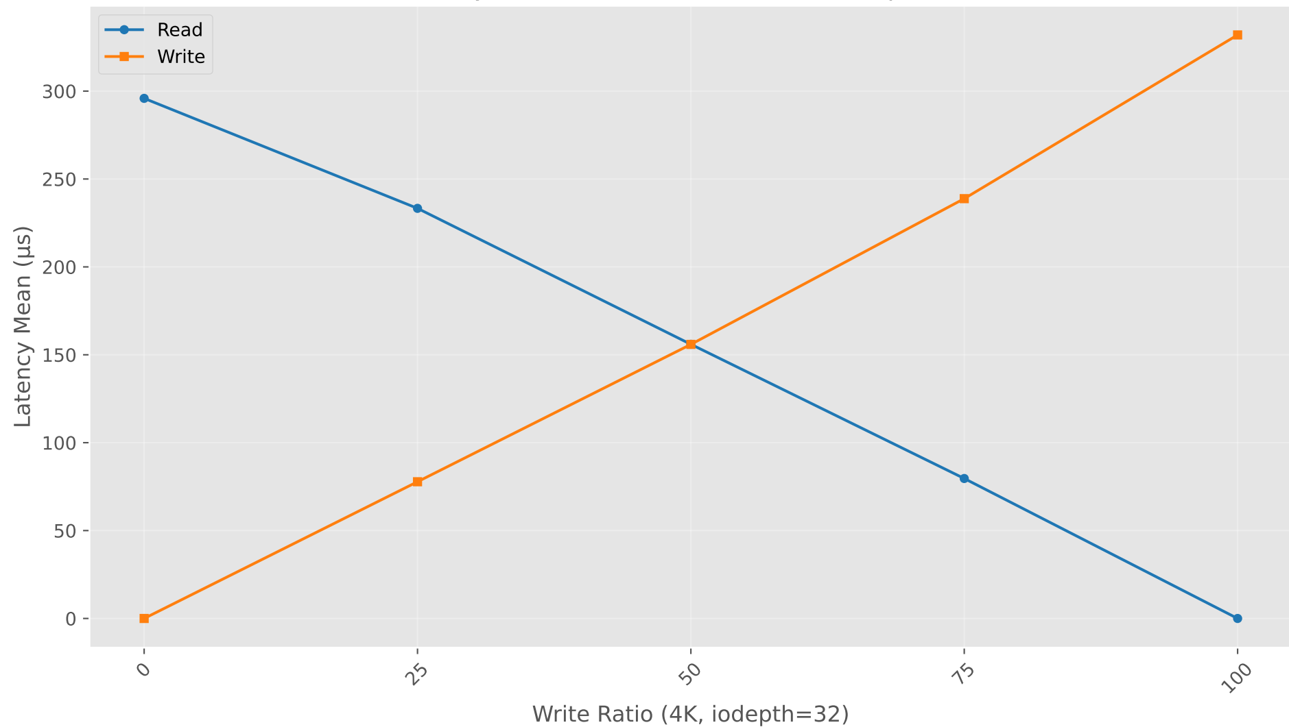
Latency Mean vs Write Ratio (4K, iodepth=32)
